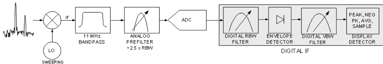
Figure 7. This block diagram of a signal analyzer IF section shows the position of the analog prefilter. It and the bandpass filter can be used to attenuate out-of-band signals and avoid ADC overload, allowing the ADC input range to be set to a lower value and improving sensitivity.
