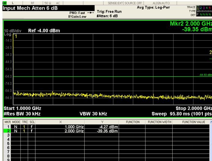
Figure A5. Reducing the stop frequency by RBW/2 removes the second harmonic from the measurement. The attenuation and measured frequency span are now optimized for spurious measurements and limit testing will show failures due only to spurious signals. Note that the actual stop frequency of 1.999985 GHz is rounded to 2.0000 GHz in the display.
