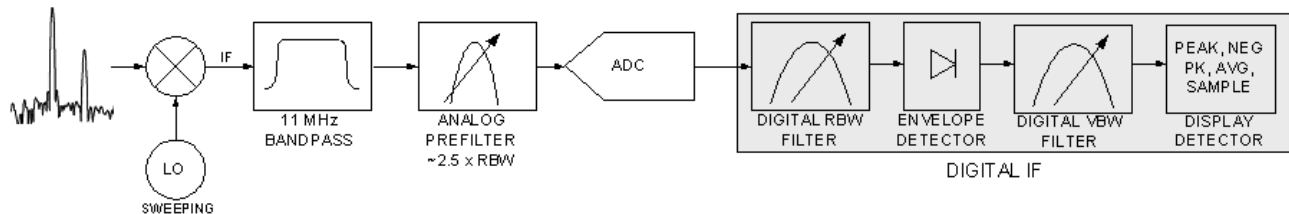
Figure A3. The analog prefilter and the bandpass filter can be used to attenuate out-of-band signals and avoid ADC overload, allowing the ADC input range to be set to a lower value and improving sensitivity.
