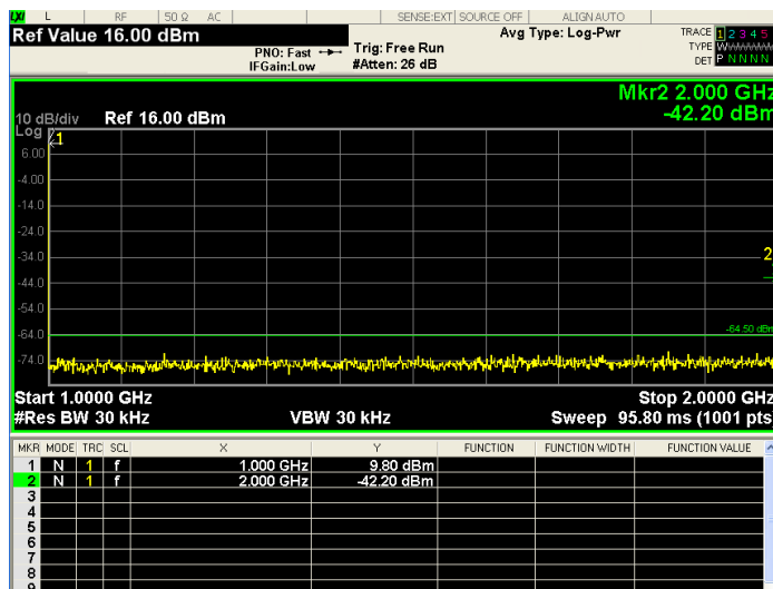
Figure A1. With the indicated frequency and attenuation settings, the measurement will fail the spurious test limit. Also, because the attenuation is not optimized for measuring spurious signals, none will be found. The analyzer was set in 'accuracy' sweep time rules for this measurement. 'Accuracy' sweep time rules provide warranted measurements at the cost of slower sweep. Fast sweep greatly improves sweep speed in 'accuracy' sweep time rules also. See X-series analyzer specification guides for more information.
